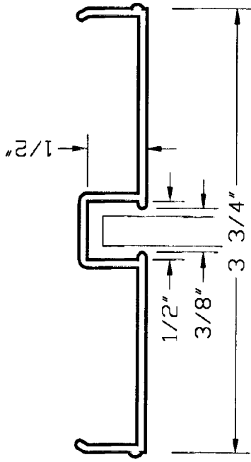
○ ECLIPSE ALUMINUM 3-3/4" NEW GLAZING SNAP-IN DETAIL
