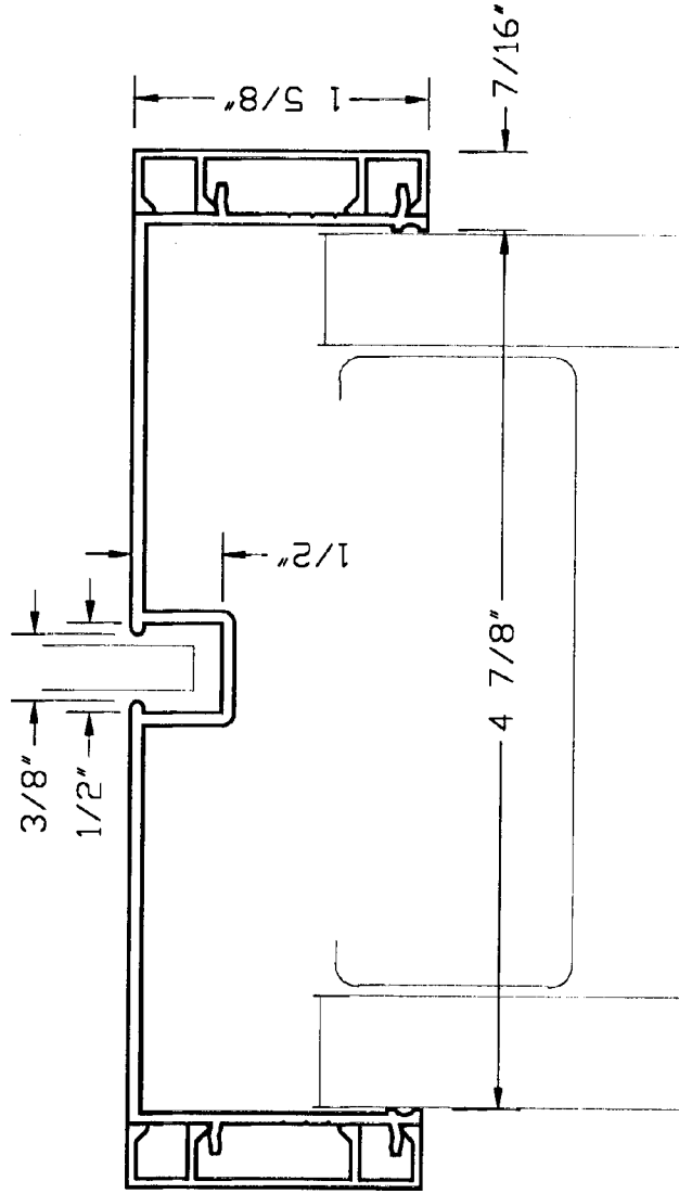
ECLIPSE ALUMINUM 4-7/8" FLUSH TRIM STYLE GLAZING RAIL
