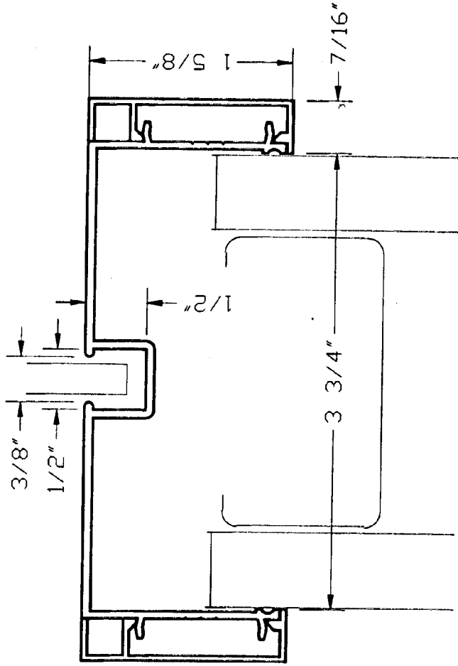
ECLIPSE ALUMINUM 3-3/4" FLUSH TRIM STYLE GLAZING RAIL
