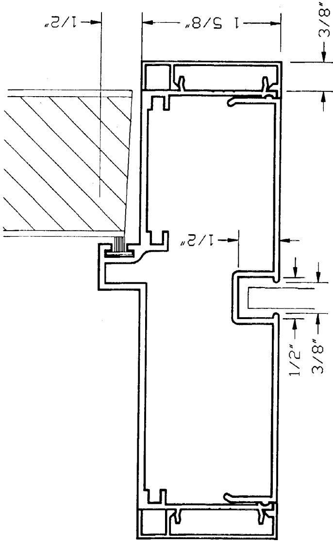
ECLIPSE ALUMINUM 4-7/8" FLUSH TRIM STYLE SIDELITE MULLION
