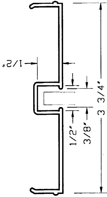
ECLIPSE ALUMINUM 3-3/4" GLAZING SNAP-IN DETAIL
